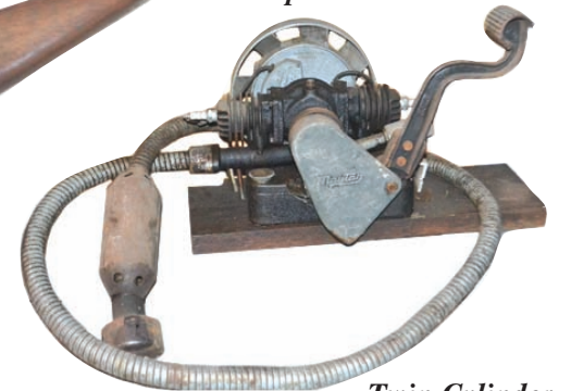
Twin Cylinder Maytag motor with exhaust.
